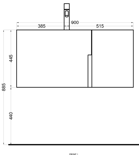
FRONT 1
