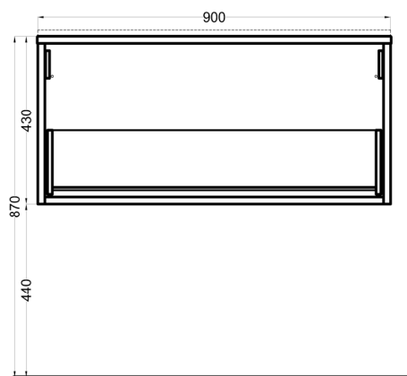
FRONT SECTION
