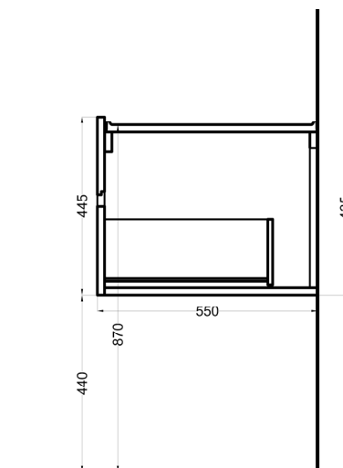
SIDE SECTION
