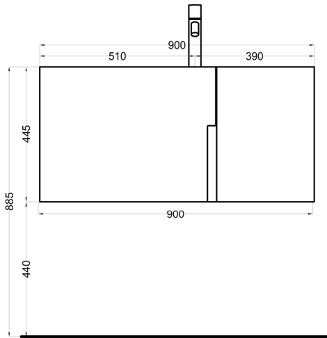
FRONT 2
