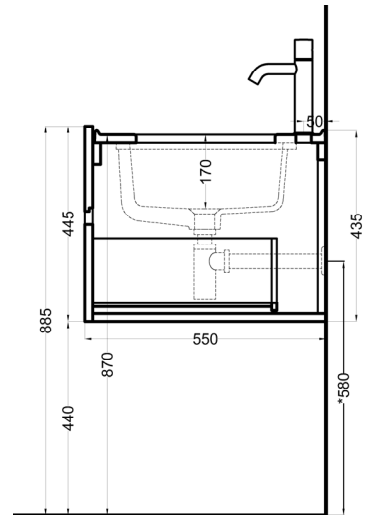
SIDE SECTION
