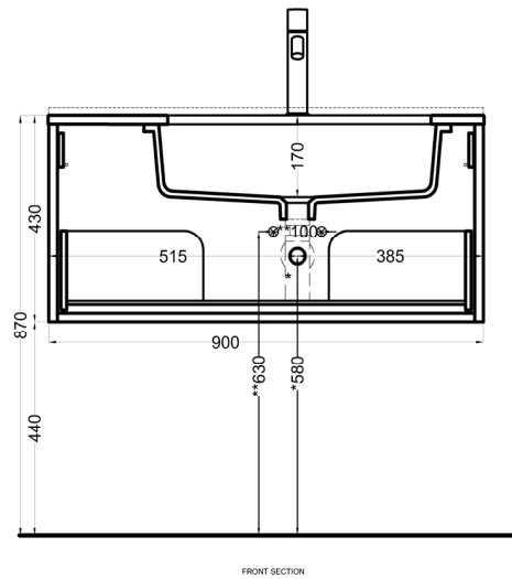
FRONT SECTION
