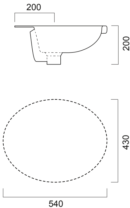
Dima del foro sul piano On top hole for washbasin fitting
